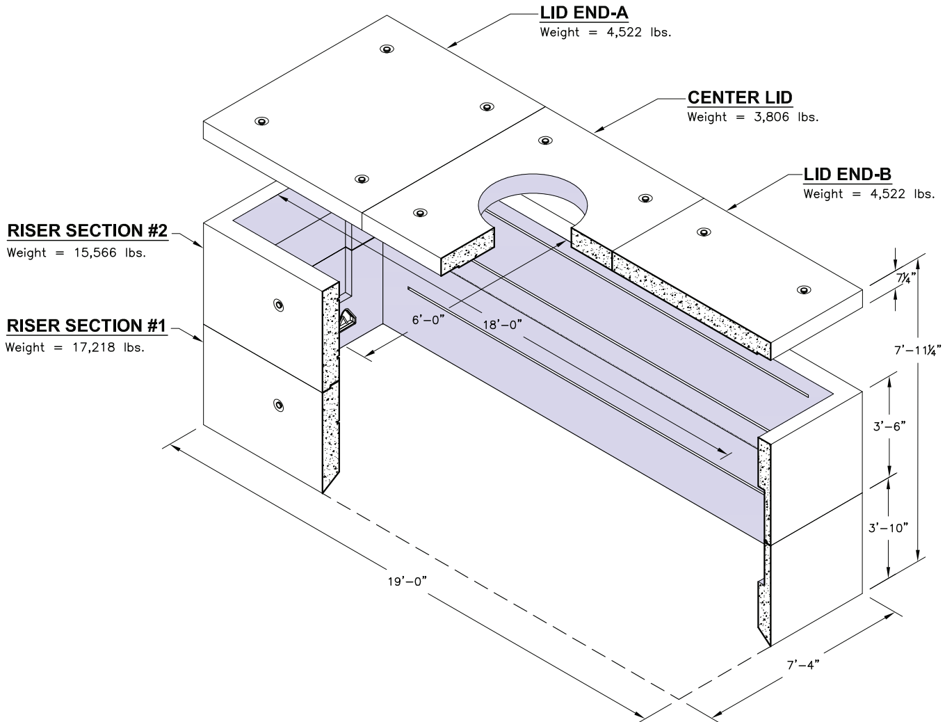
Electrical Vault Kit Components
