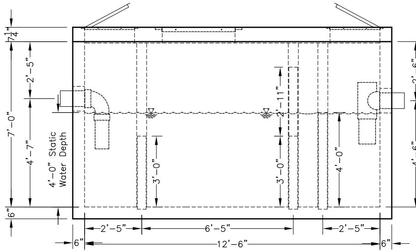
Elevation View
