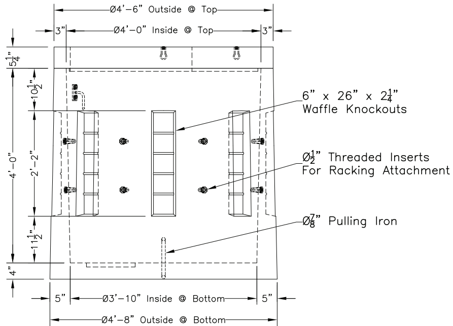
Elevation View
