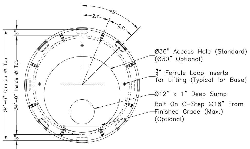
Plan View
