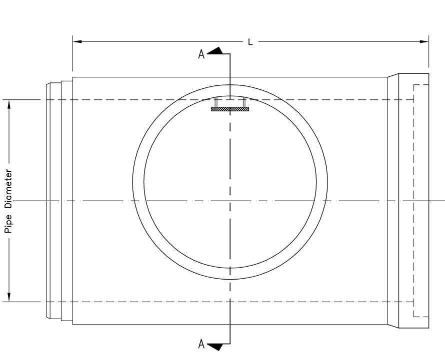
Plan View
