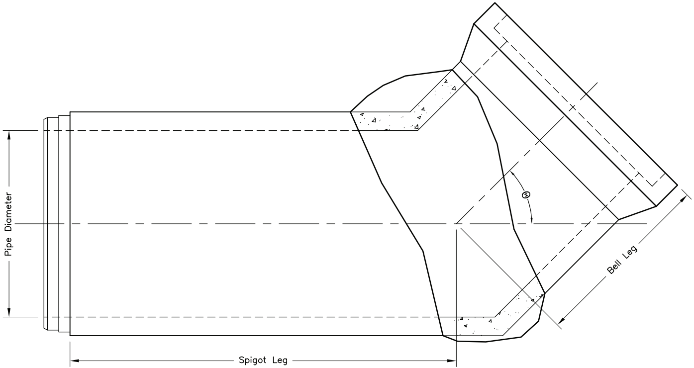
Standard RCP Elbow with Bell-Top View
