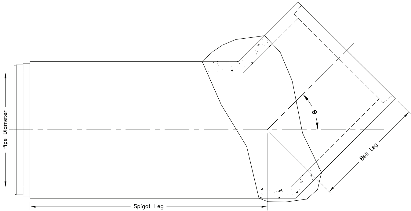
Standard RCP Elbow without Bell-Top View
