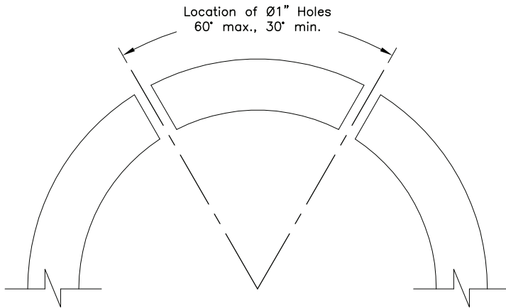
Fastener Spacing End View
