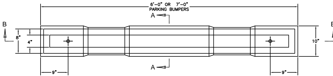
PLAN VIEW
