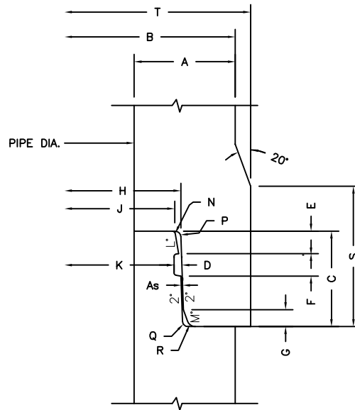
MODIFIED "BABY" BELL JOINT DETAIL 36" & 42" DIA. ONLY
