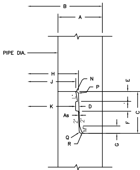
STANDARD JOINT DETAIL
