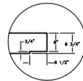
TYP. LID JOINT DETAIL
