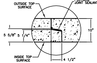
JOINT DETAIL FOR WALLS 10" AND 12"
