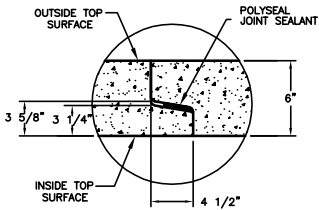
JOINT DETAIL FOR WALLS 6" AND 8" THICK
