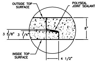
JOINT DETAIL FOR WALLS 6" AND 8" THICK
