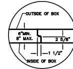
JOINT DETAIL FOR WALLS 6" AND 8" THICK
