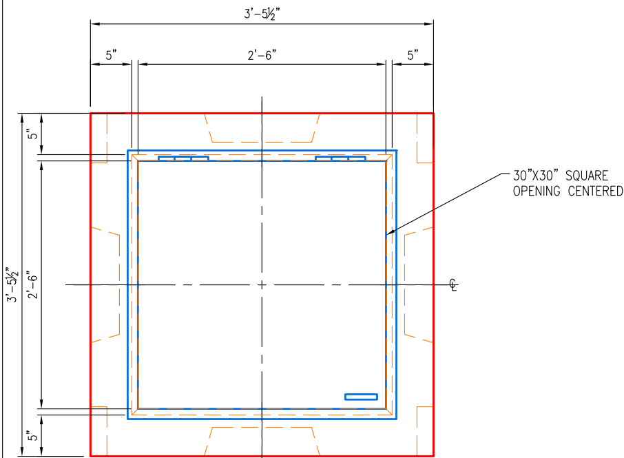
PLAN VIEW SCALE: 3/4" = 1'-0"
