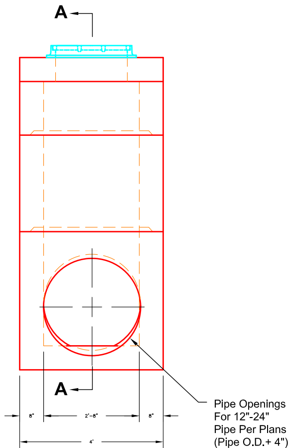
ELEVATION VIEW
