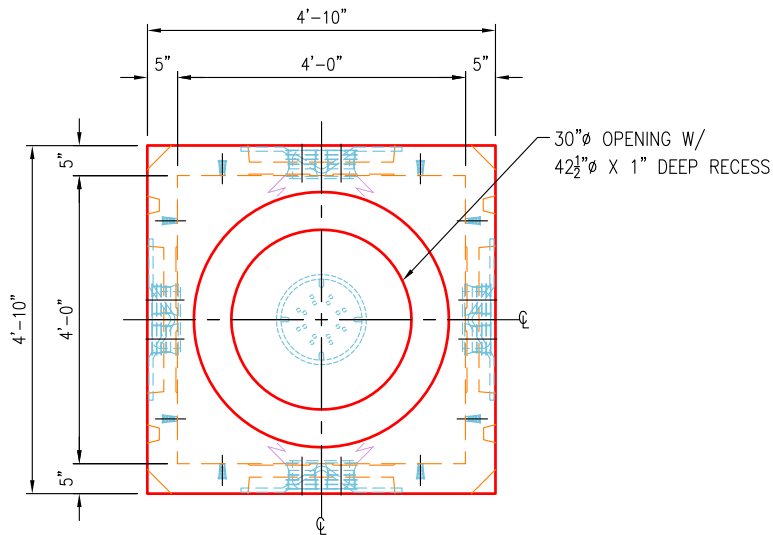
PLAN VIEW SCALE: 3/8" = 1'-0"
