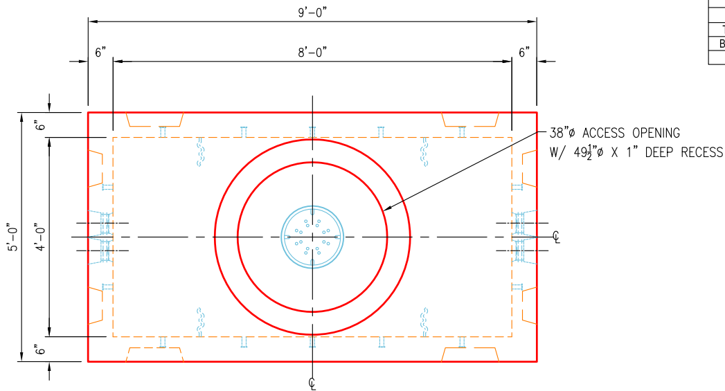
PLAN VIEW SCALE: 3/8" = 1'-0"
