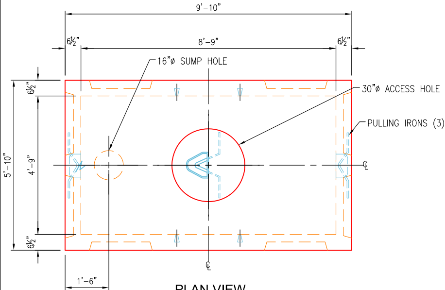
PLAN VIEW SCALE: 5/16" = 1'-0"
