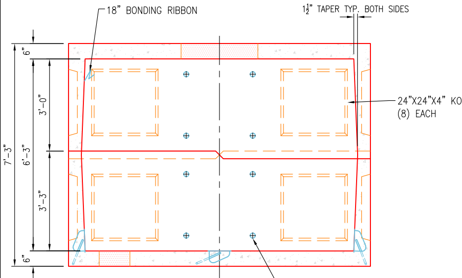
SIDE VIEW SCALE: 5/16" = 1'-0"
