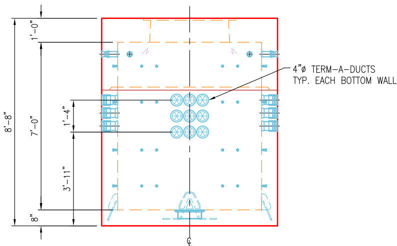
SIDE VIEW SCALE: 1/4" = 1'-0"
