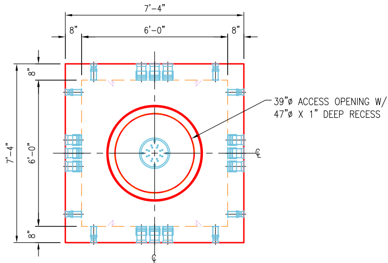
PLAN VIEW SCALE: 1/4" = 1'-0"
