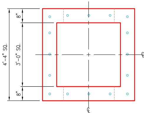
PLAN VIEW SCALE: 3/8" = 1'-0"
