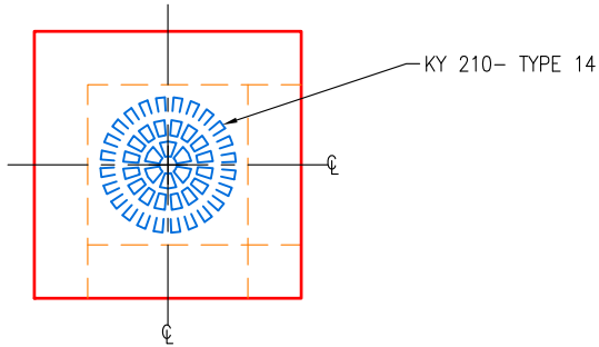
PLAN VIEW SCALE: 3/8" = 1'-0"
