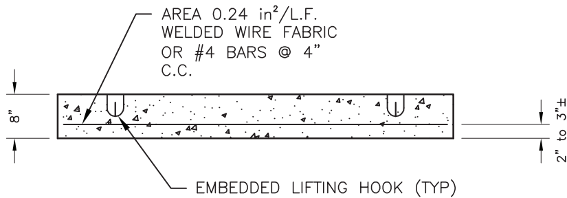
SECTION VIEW
