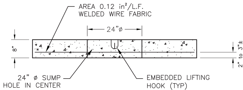
SECTION VIEW
