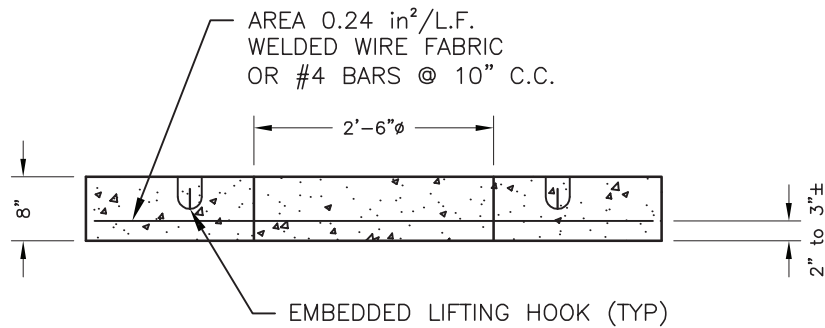
SECTION VIEW
