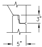
JOINT DETAIL
