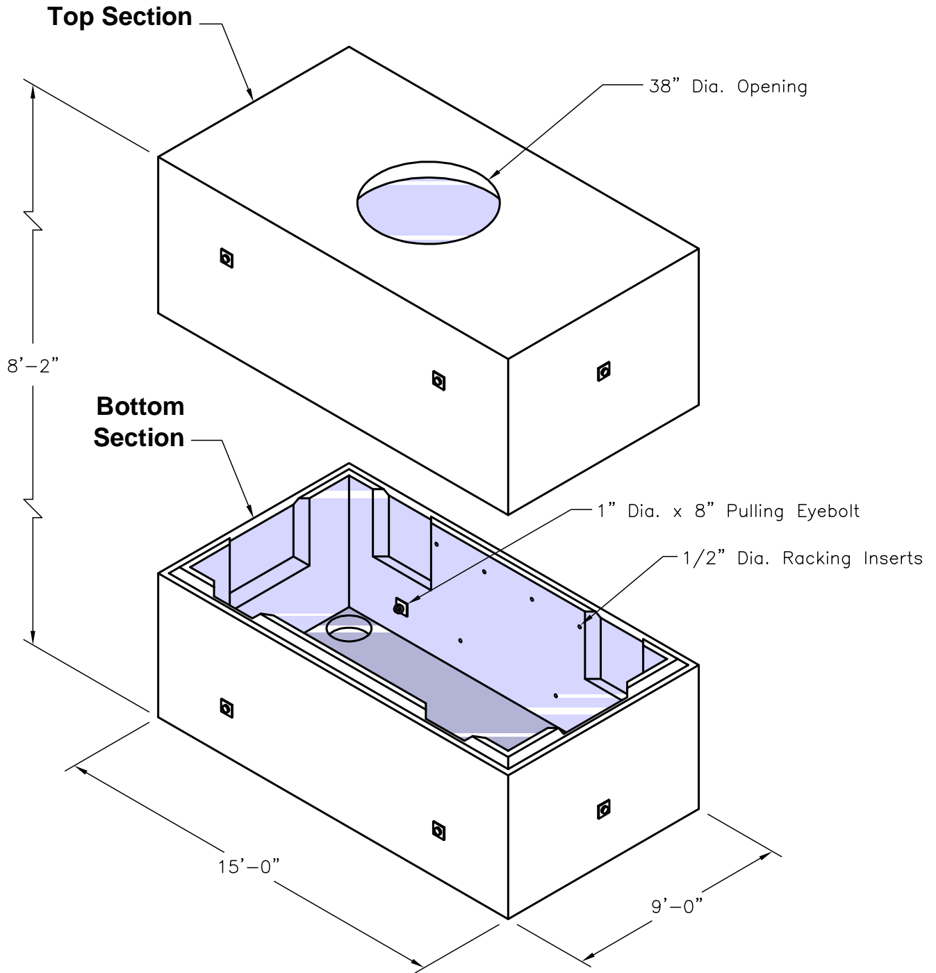
ISOMETRIC VIEW
