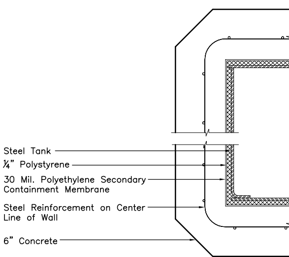
SECTION DETAIL
