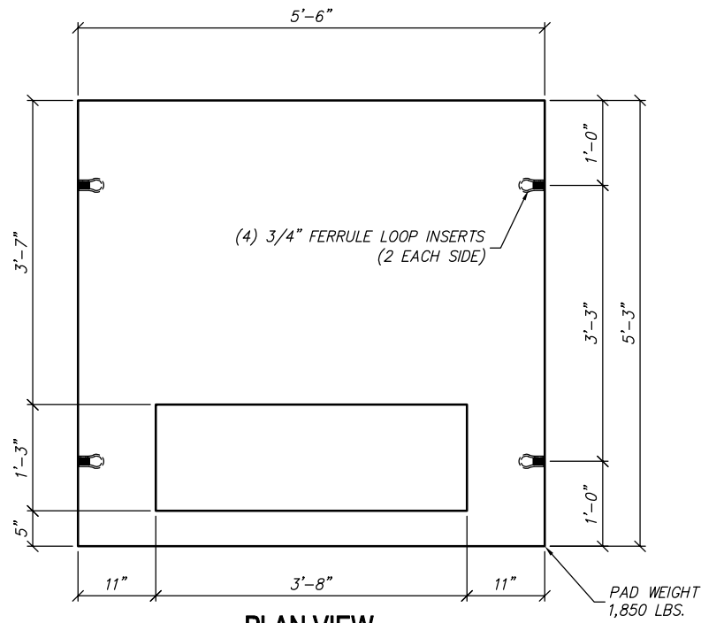
PLAN VIEW SCALE: 1/2" = 1'-0"
