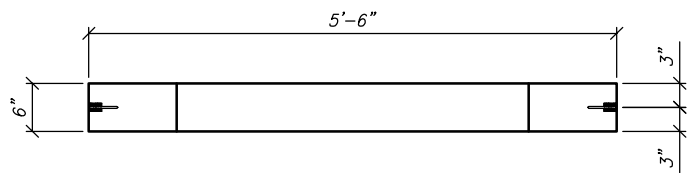
SECTION VIEW SCALE: 1/2" = 1'-0"
