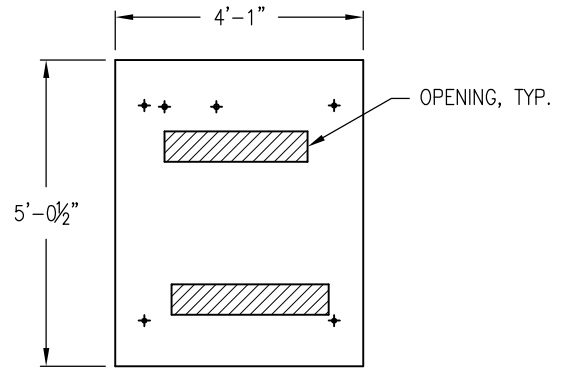
PMH-4 (25 Kv) CODE NO.: 04-0995
