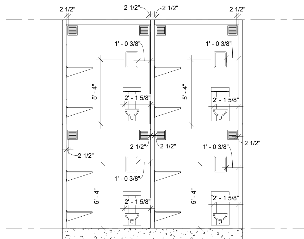
⑤ LAVATORY, MIRROR AND HVAC GRATES 1/4" = 1'-0"
