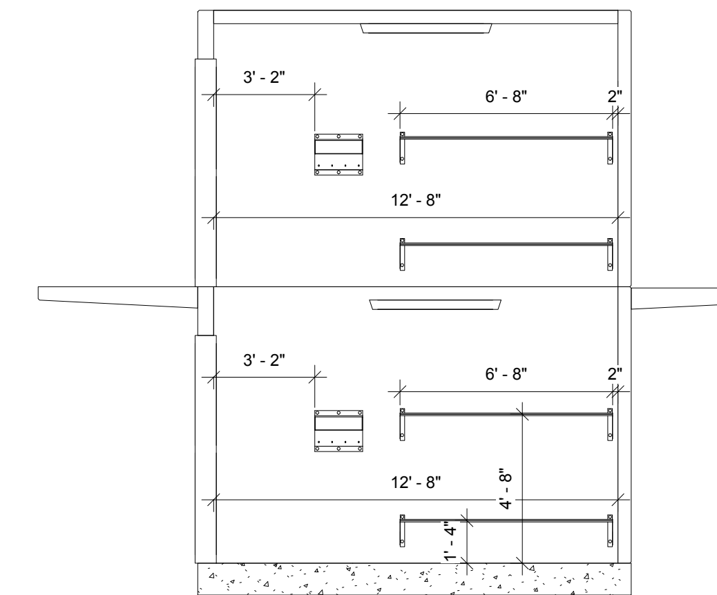
③ BED AND SHELF LOCATION 1/4" = 1'-0"
