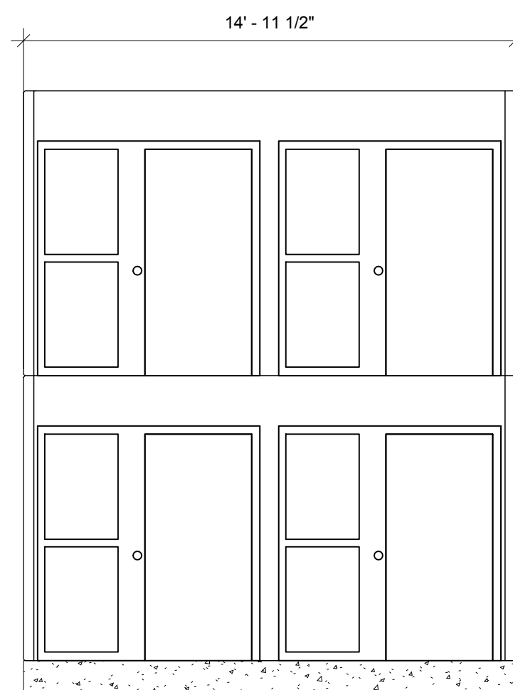
④ CELL DOOR AND WINDOW 1/4" = 1'-0"
