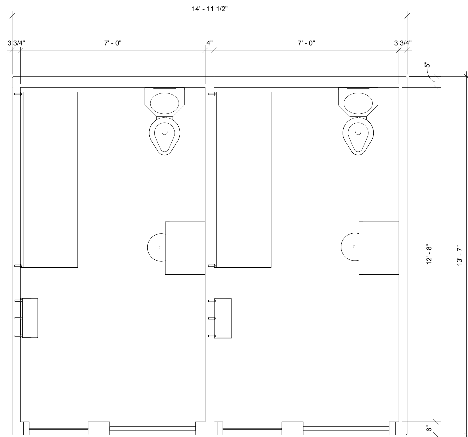
① PLAN VIEW 1/2" = 1'-0"
