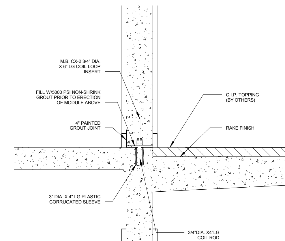
⑦ CELL TO CELL CONNECTION 1" = 1'-0"
