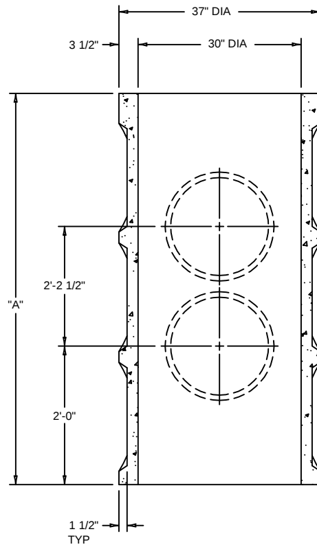
SECTION "X"-"X"
