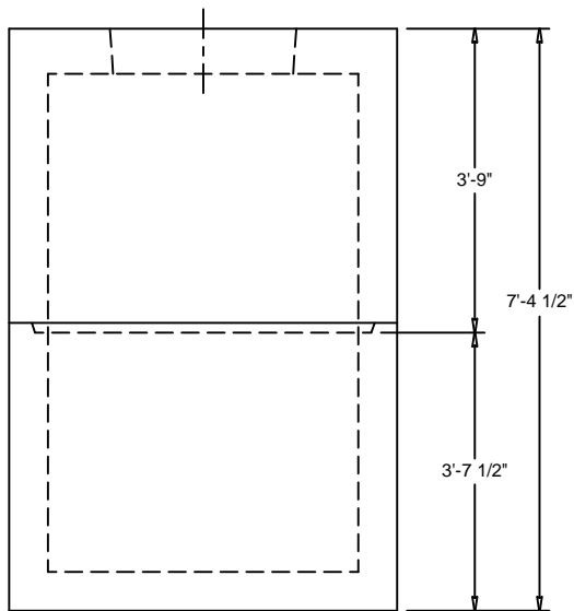
VIEW "X"-"X"
