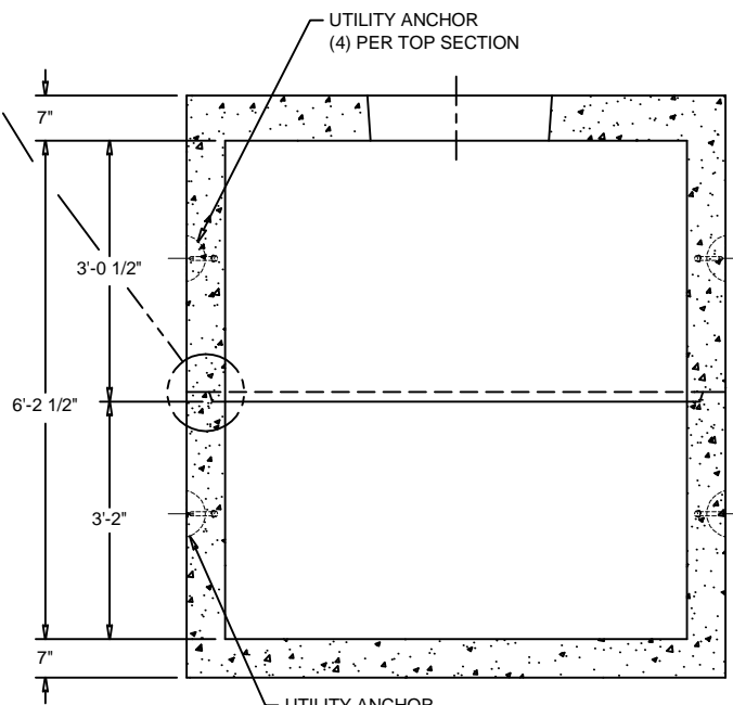
SECTION "Y"-"Y"
