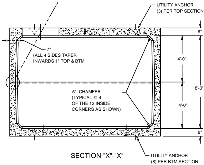
JOINT DETAIL SHOWN OPEN FOR CLARITY
