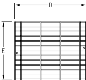
TRAFFIC GRATE PLAN VIEW
