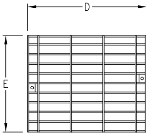
PEDESTRIAN GRATE PLAN VIEW
