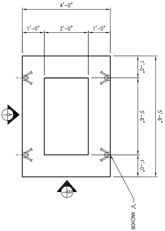
PLAN VIEW SCALE: 3/8" = 1'-0"
