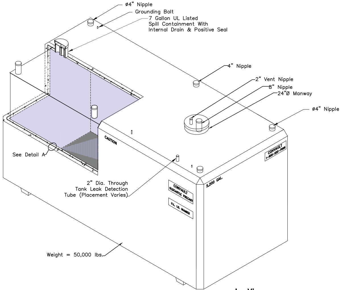
Iso View For Reference Only
