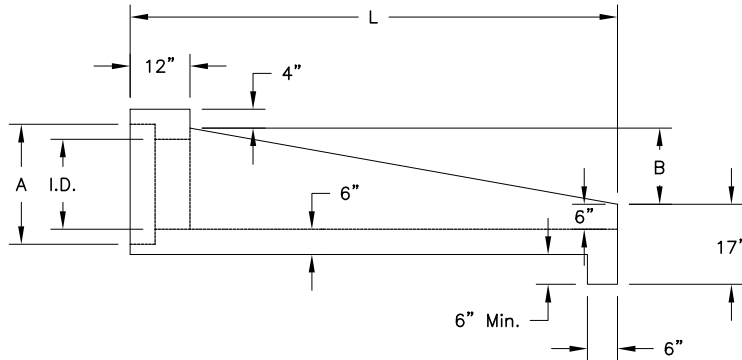
ELEVATION VIEW
