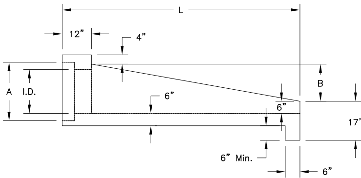
ELEVATION VIEW
