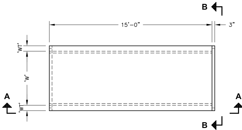
PLAN VIEW
