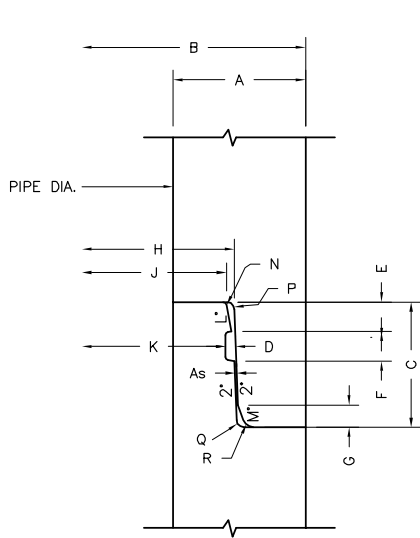
STANDARD JOINT DETAIL
