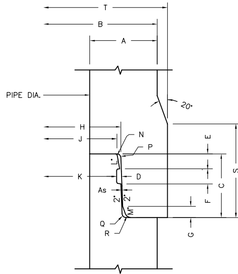
MODIFIED "BABY" BELL JOINT DETAIL 36" & 42" DIA. ONLY
