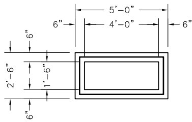
18" X 48" BASE / RISER PLAN VIEW
