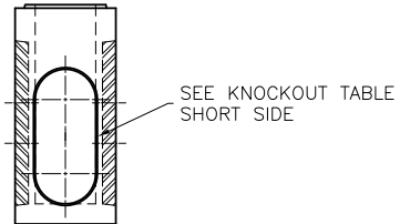
18" X 48" BASE END VIEW
