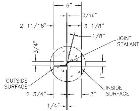
JOINT DETAIL
