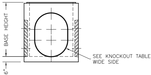
18" X 48" BASE ELEVATION VIEW
