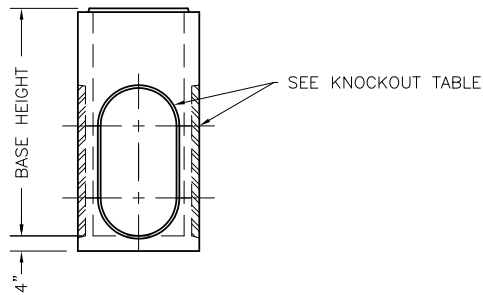
2'x2' CATCH BASIN BASE ELEVATION VIEW
