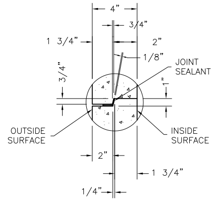
JOINT DETAIL
