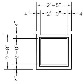
2'x2' CATCH BASIN PLAN VIEW
