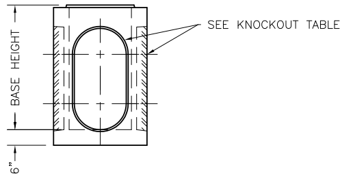
2'x2' CATCH BASIN BASE ELEVATION VIEW
