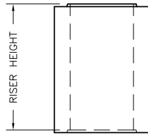
2'x2' CATCH BASIN RISER ELEVATION VIEW
