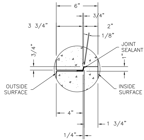
JOINT DETAIL
