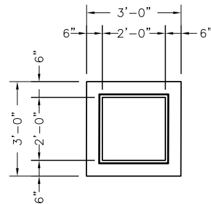
2'x2' CATCH BASIN PLAN VIEW
