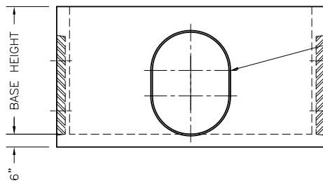
2' X 9'-6" CATCH BASIN SIDE ELEVATION
