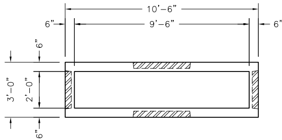
2' X 9'-6" CATCH BASIN PLAN VIEW
