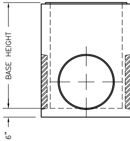
4'x4' CATCH BASIN BASE ELEVATION VIEW
