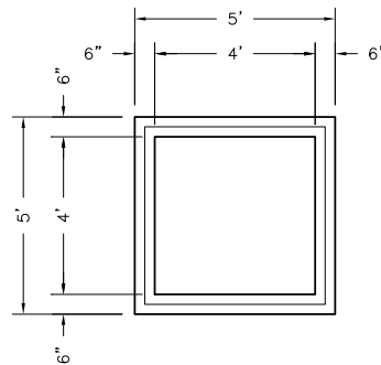
4'x4' CATCH BASIN BASE / RISER PLAN VIEW
