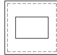
4'x4' CATCH BASIN LID PLAN VIEW 2'x3' OPENING CENTER/OFFSET 18"x48" OPENING CENTER/OFFSET
