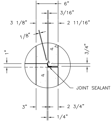
JOINT DETAIL
