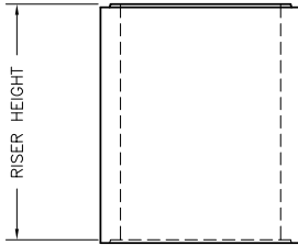
4'x4' CATCH BASIN RISER ELEVATION VIEW
