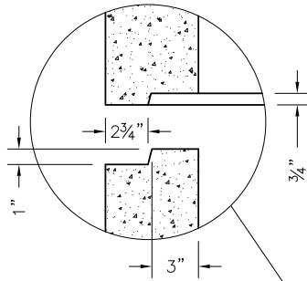
JOINT DETAIL
