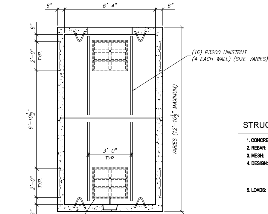
SECTION VIEW
