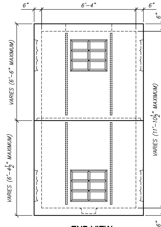
END VIEW
