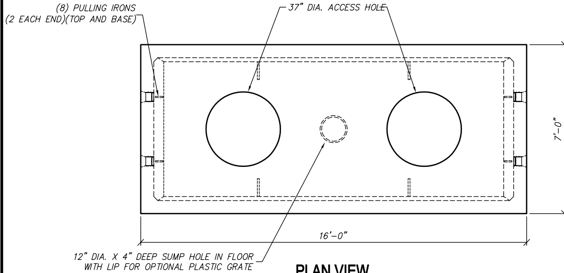
PLAN VIEW SCALE: 1/4" = 1'-0"
