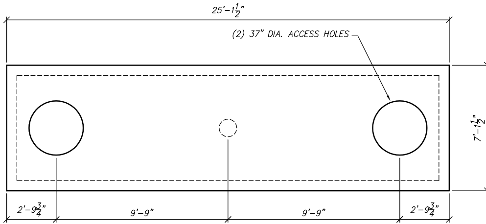
PLAN VIEW SCALE: 3/16" = 1'-0"
