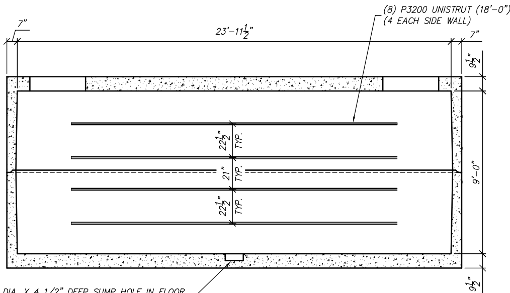
SECTION VIEW SCALE: 3/16" = 1'-0"
