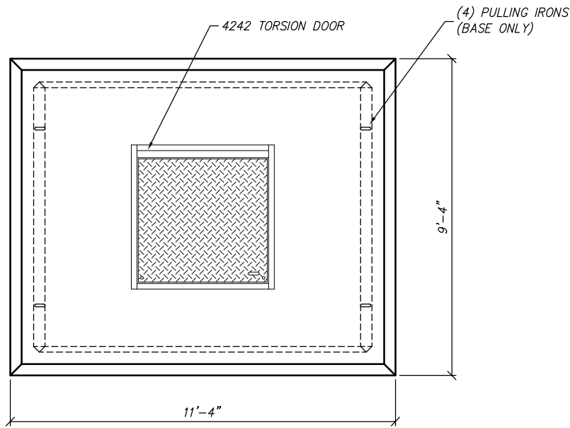
PLAN VIEW SCALE: 1/4" = 1'-0"
