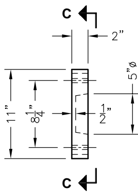
PLAN VIEW END CAP
