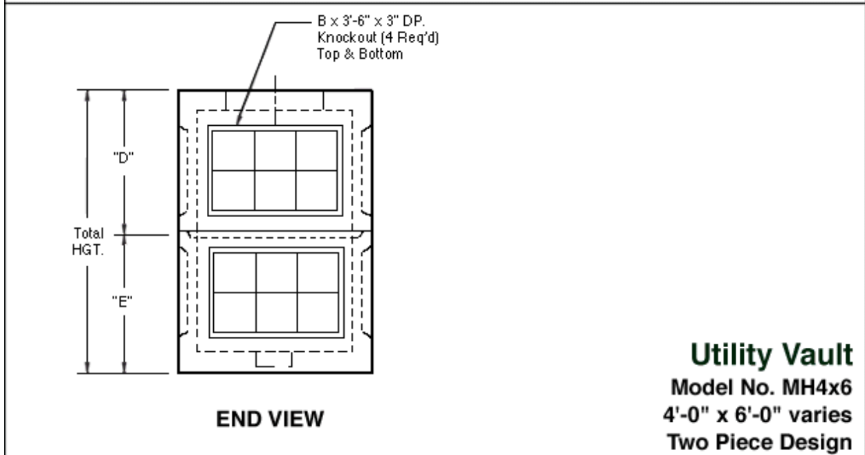
Utility Vault Model No. MH4x6 4'-0" x 6'-0" varies Two Piece Design
