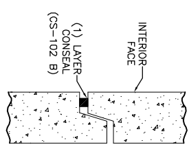
TYPICAL JOINT DETAIL (SCALE: NTS)
